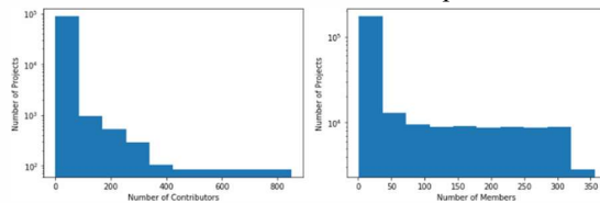
Figure 3. Distribution of number of contributors (left) and number of members (right) of projects.
