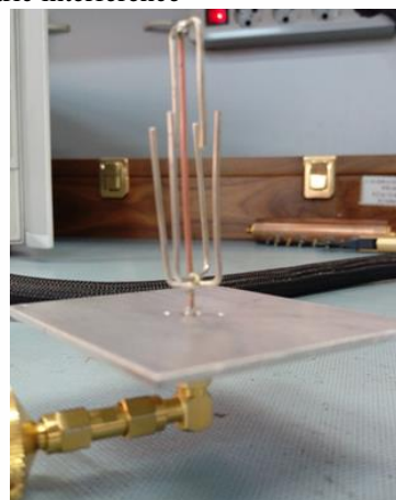
Figure 2. Fabricated multi-band monopole antenna.
