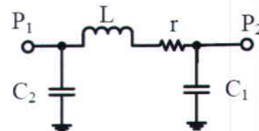
Fig.10 simplified symmetric Inductor Model
