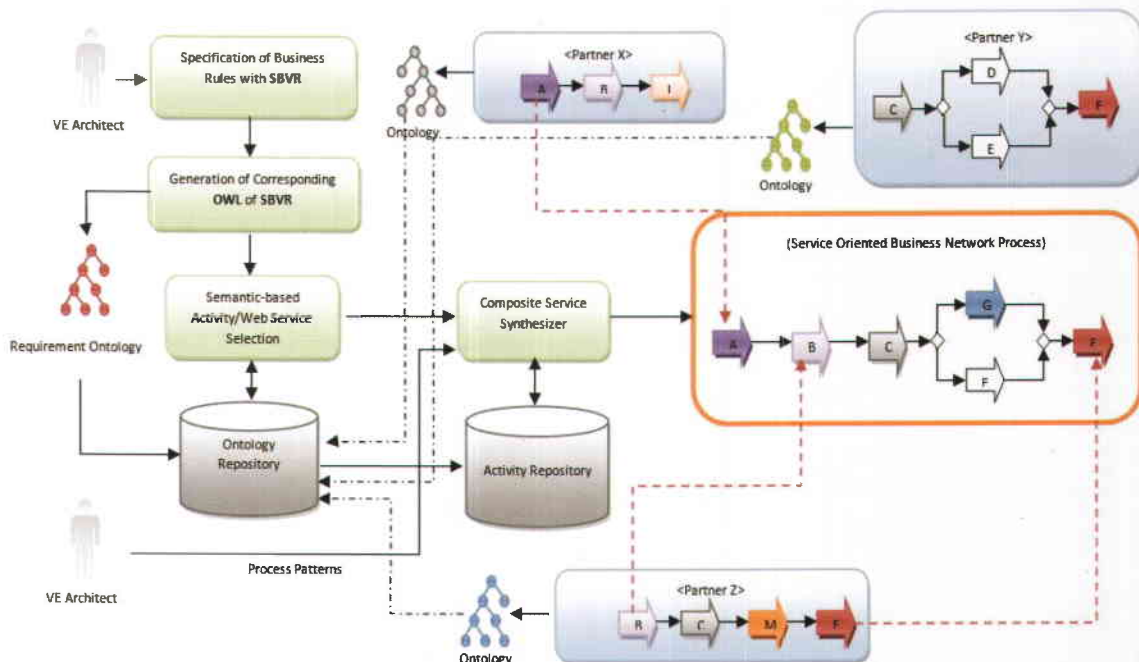
Figure 5. Architecture of prototype
