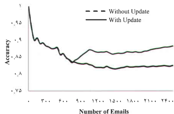
Figure 7. Effect of concept drift detection on accuracy with block length 300
