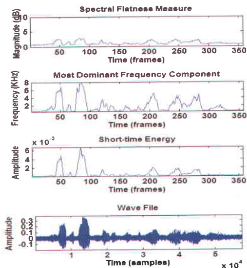
Fig. 6. Feature values for a speech signal corrupted with White noise at 5 dB SNR. Noises are extracted from NOISEX-92 corpus.
