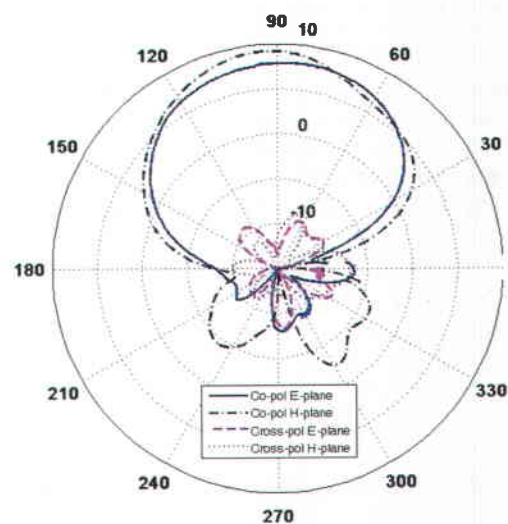
Figure 13. Measurement of co- and cross-polarization radiation patterns at 1030MHz.
