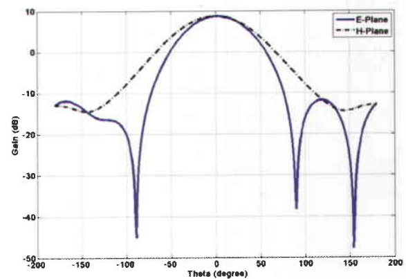
Figure 3. E- and H-plane radiation patterns at 1030MHz simulated by IE3D.
