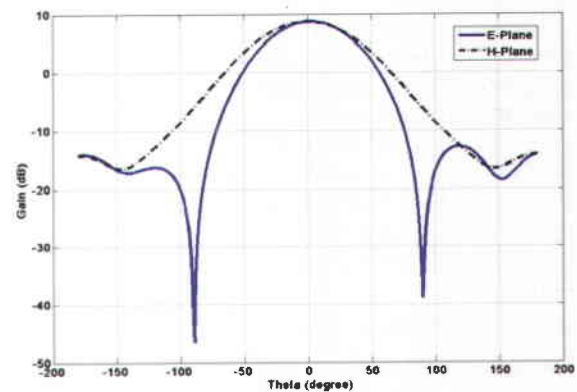
Figure 4. E- and H-plane radiation patterns at 1090MHz simulated by IE3D.
