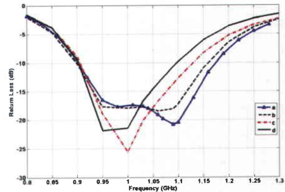
Figure 2 Return losses of four structures simulated by IE3D.
