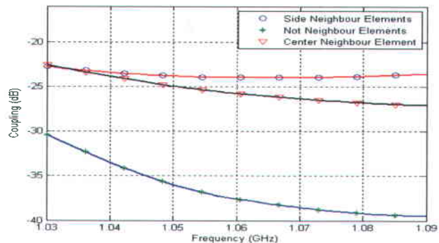
Figure 6. Coupling between center and side elements in an 8 \times 1 array.
