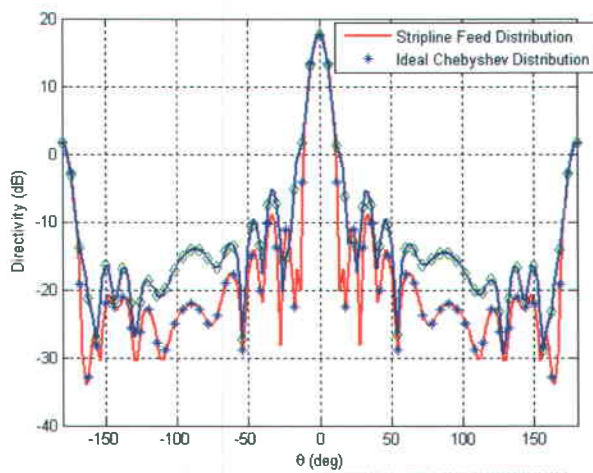
Figure 10. Sum pattern at 1030MHz for the simulation.
