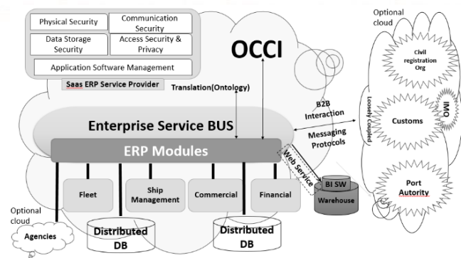
Fig. 2: Proposed Framework
