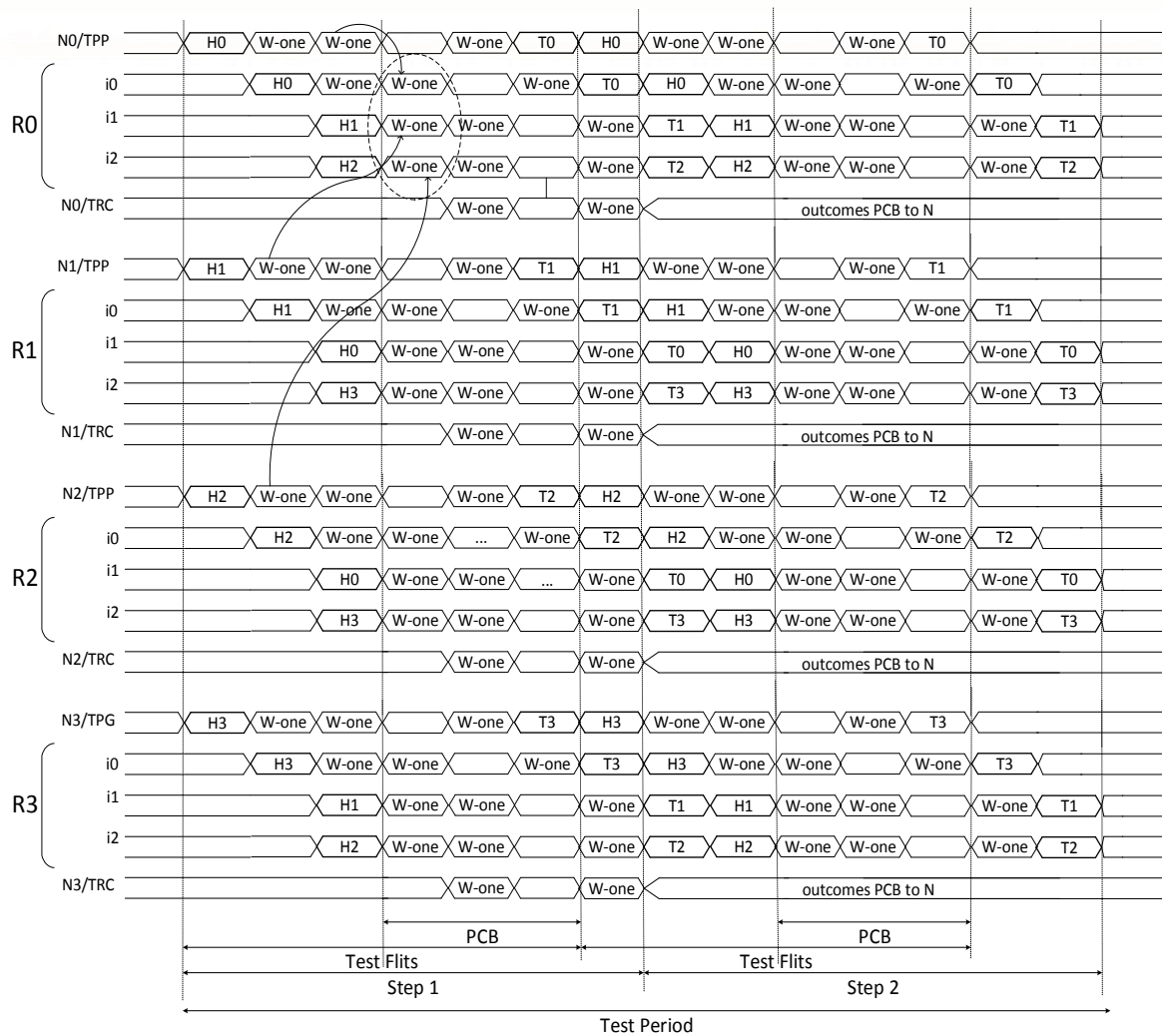
Fig.7. OSDTM timing
