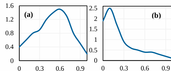
Figure 4. Aggregate distribution of attention weight of words good (a) and bad (b) on test split of SST1 dataset.
