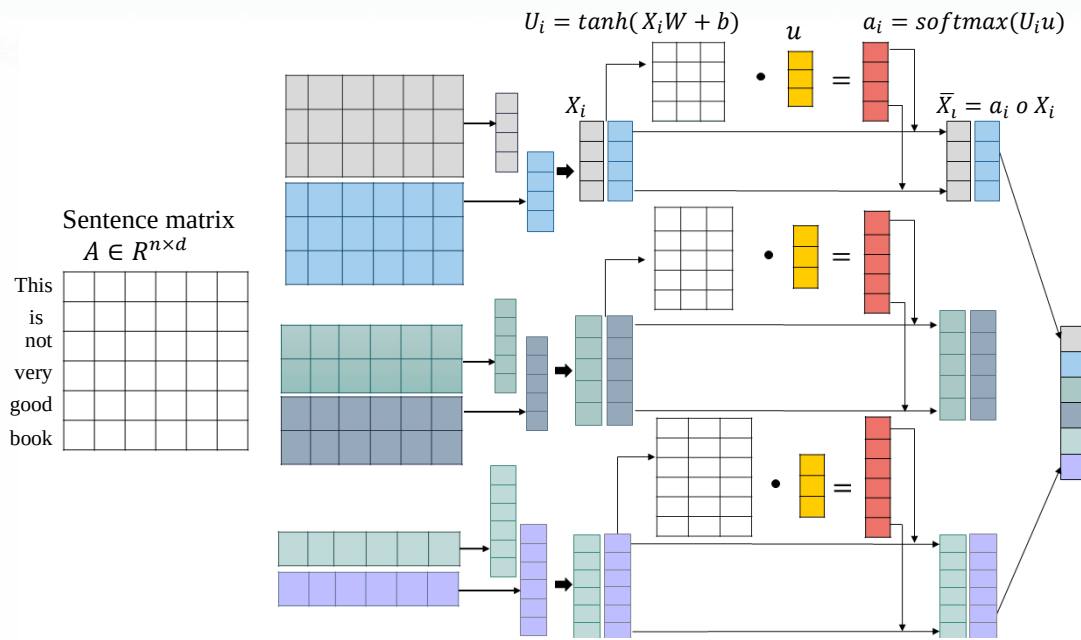
Figure 2. Structure of the convolutional neural network integrated with attention layer.
