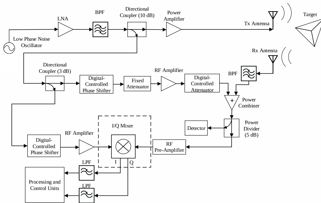
Figure 1. Complete block diagram of the MLDS.
