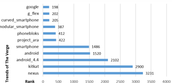
Figure 13. Kumar and Jaiswal [37] predicted trends for 1000 iterations.
