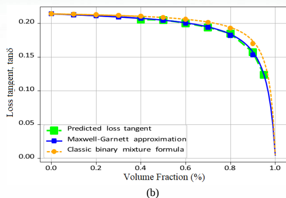
Fig 13. (a) The Relative permittivity (b) Loss tangent of the mixture of water and cyclohexane as a function of the volume.
