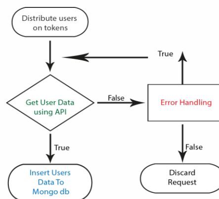
Figure 5. Data gathering flow chart
