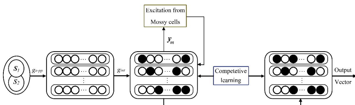
Figure 6. Structure of the proposed network based on Dentate Gyrus of hippocampus
