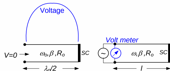
Figure 1. Half wavelength method for cable's permittivity extraction.
