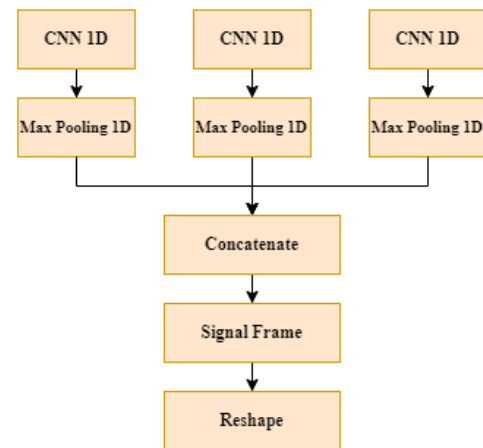
Fig. 1. Feature Extraction
