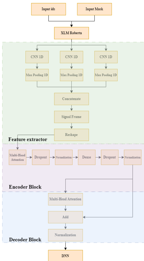
Fig. 2. Model Architecture
