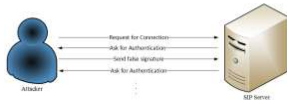
Fig. 1- A sample authentication based attack
