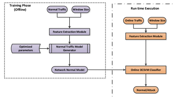
Fig. 7 - OCSVM based classification used for performance evaluation of engineered feature sets
