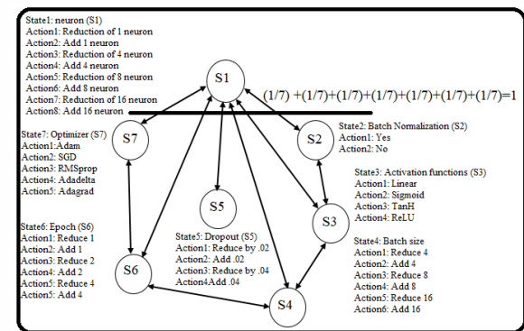
Figure 3. State and action in later stages.
