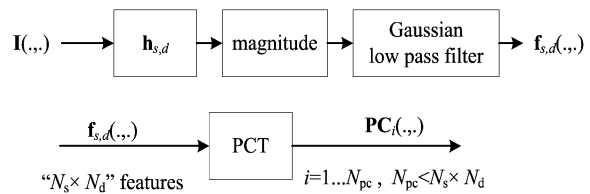
Fig 4. Gabor features extraction process. Refer to context for details.
