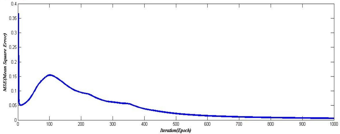
Fig. 7. MSE in each epoch for CT-PCA optimized-MLP using ICA method
