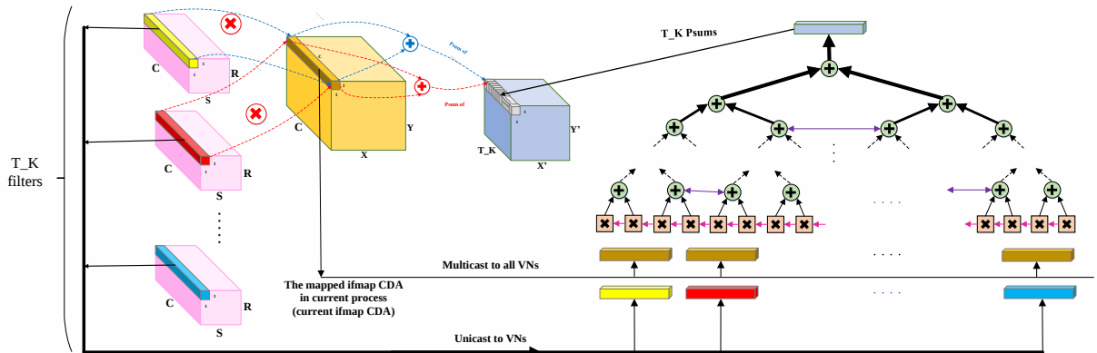
Figure 6. The designed CPC-based dataflow to test the FUCA (designed as CDS)
