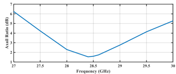
Figure 9. Axial ratio of the antenna versus frequency.
