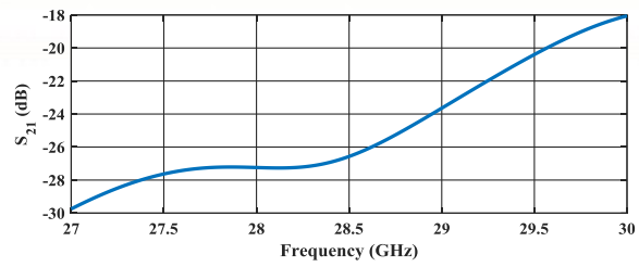
Figure 8. The S_{21} (isolation) of the antenna over frequency.
