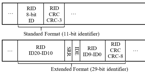
Fig. 5. MRMC+ ID Format
