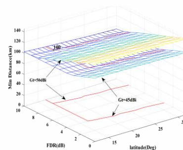
Figure 9. The curve of FDR versus latitude in order to maintain a minimum allowable distance of 100 kilometers for G_t=45dBi and G_t=50dBi .
