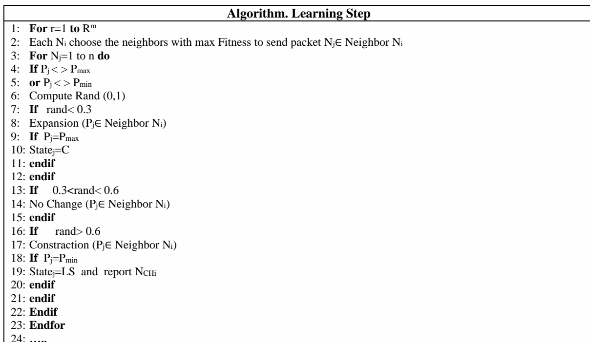
Figure 3. Simi-code of learning automata
