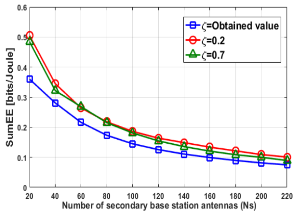
Figure 4. Sum energy efficiency (sumEE) of the secondary system versus the number of secondary base station antennas ( N_s ) in different values of energy allocation ratio of the jammer ( \zeta ) (with \rho=0.5 and Q=10 dB).
