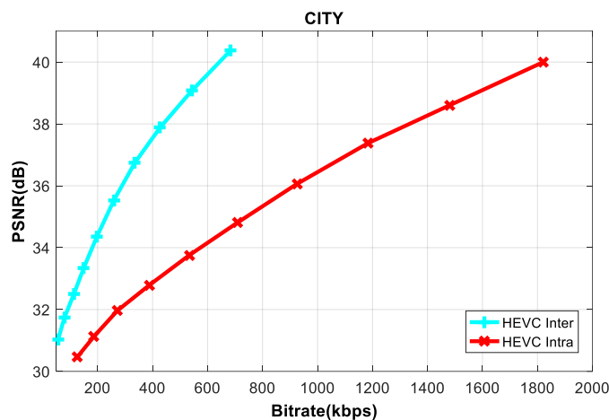
Fig. 15. Comparison of RD performance of HEVC Intra and Inter modes; "City" video sequence.
