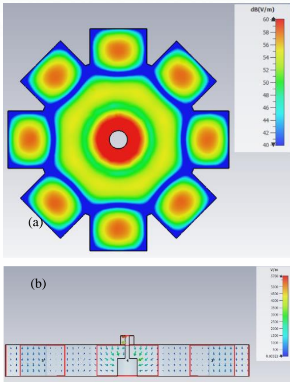
Figure 9. The simulated electric field of the proposed 8x1 radial power combiner in 12.5 GHz in top (a) and side (b) view planes.
