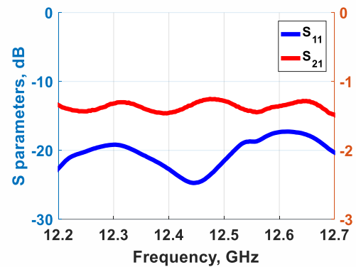
Figure 12. Measured results of the radial power combiner in back to back configuration, insertion loss (right), return loss (left).
