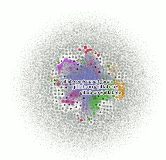
Figure 4. Project graph. Created by mono-partite projection of the user-project contribution bi-partite graph. Colors represent different modularity classes of the nodes.
