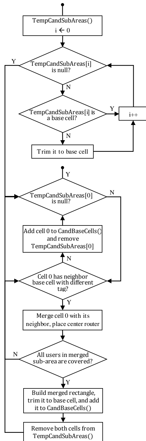
Fig. 12. Main steps of function RecombTempCandCells()
