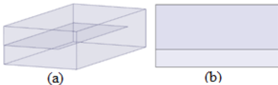
Fig. 1. Partial H-plane waveguide. (a) Side view. (b) Top view.
