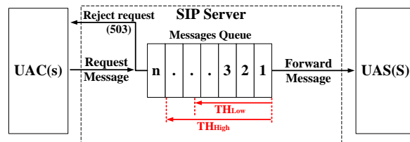
Fig. 9. Queuing structure and thresholds
